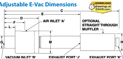
Adjustable Vacuum Generator Dimensions
