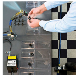
The Gen4 Model 8910 Instant Static Elimination Station removes contaminants on plastic fittings prior to packaging.
